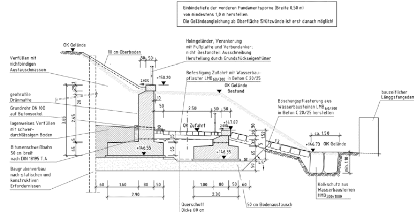
Cross section
