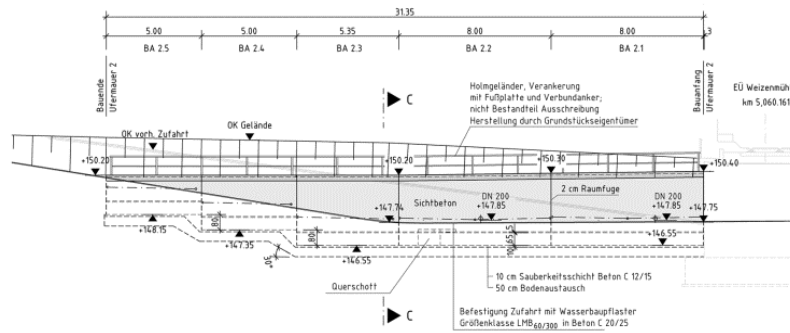
Elevation river bank 2
